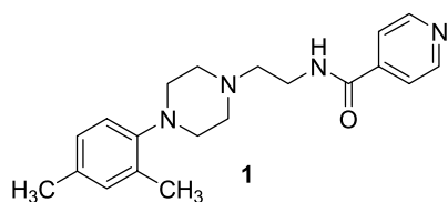
Figure 1. Pharmacophore model mapped to 1 .
