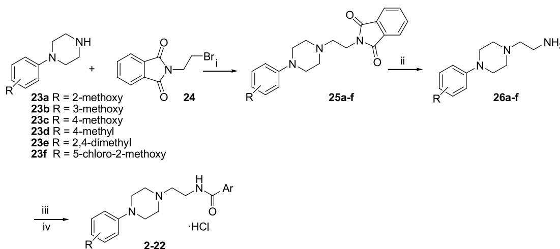
Scheme 1. Reagents and conditions: (i) Et 3 N, CH 3 CN, 100 °C; (ii) N 2 H 4 · H 2 O, EtOH, 80 °C; (iii) ArCOCl, K 2 CO 3 , CH 3 CN, 100 °C; (iv) ethanolic HCl.
